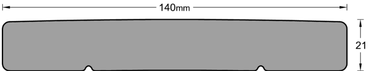
Camber Decking
