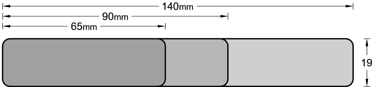
Plain Decking
