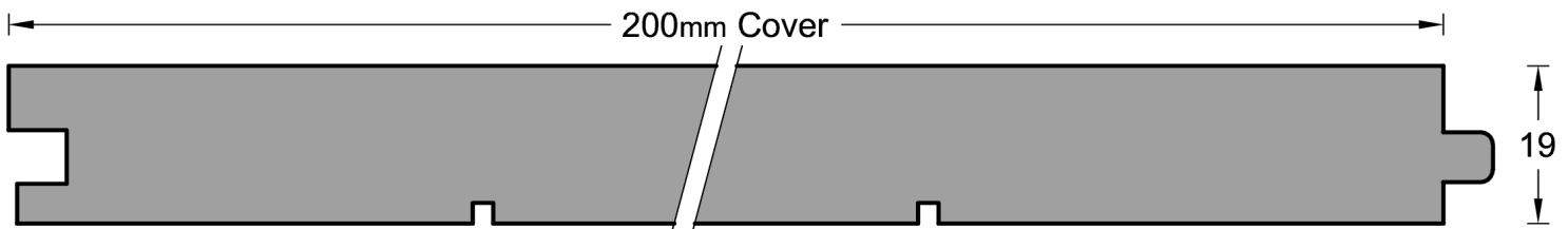
T&G Timber Flooring Profile (French Oak Only)
