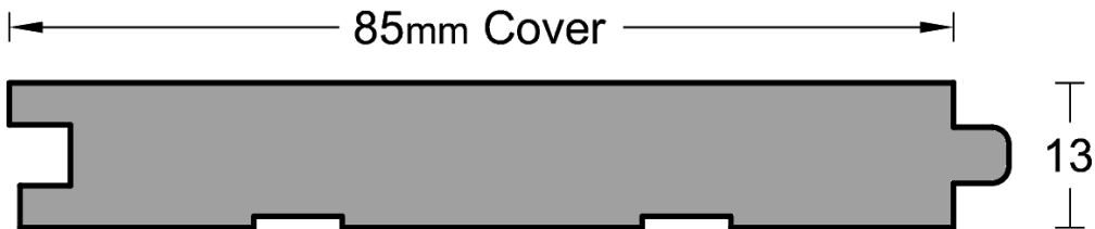
T&G Timber Flooring Overlay
