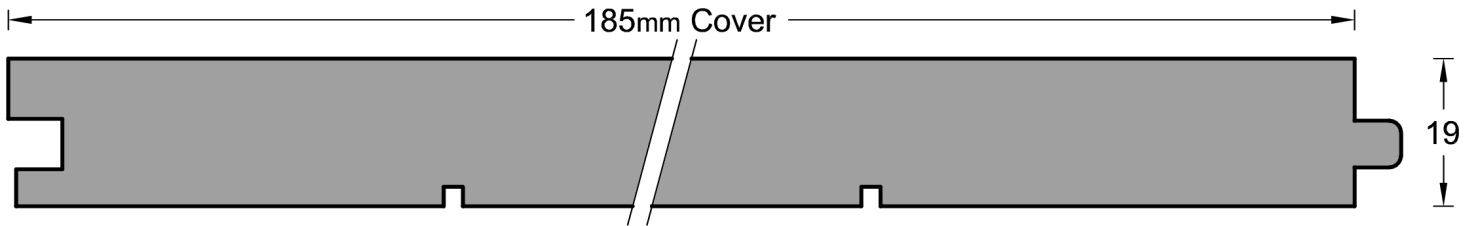
T&G Timber Flooring Profile
