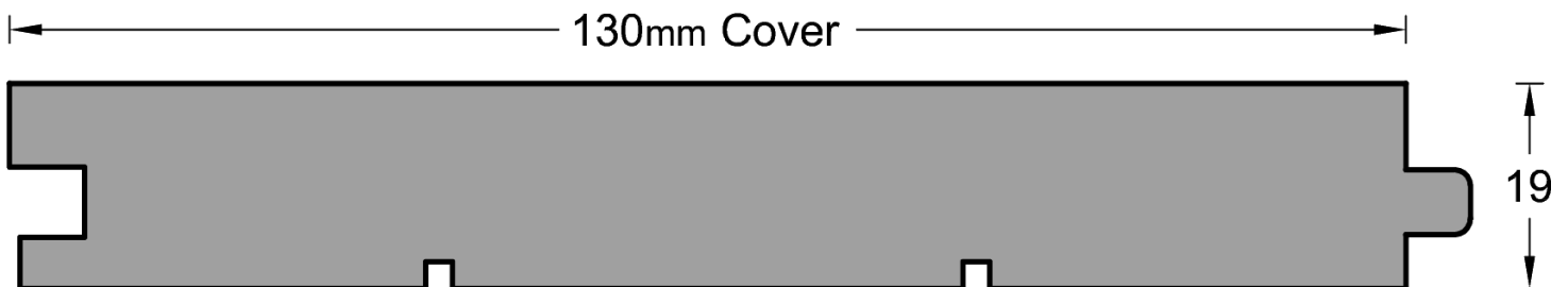
T&G Timber Flooring Profile
